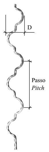
Art. 621/1 □ 12 x 12 mm D 100 mm Passo - Pitch 260 mm
