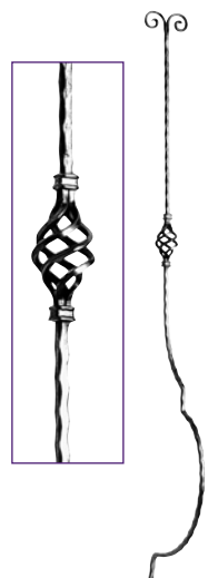
Art. 1273/17 □ 12 x 12 mm 1200 mm
