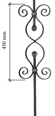
Art. 1127/3 □ 12 x 12 mm 205 x 1000 mm
