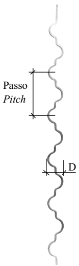
Art. 620/1 \varnothing 12 x 12 mm D = 100 mm Passo - Pitch 260 mm
