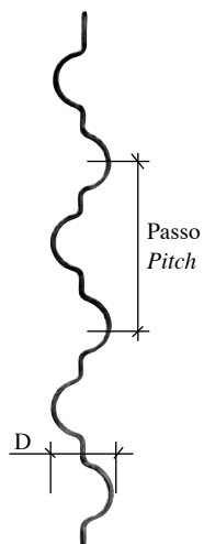
Art. 38/1 8 x 8 mm D 84 x 240 mm Passo - Pitch L 1600 mm
