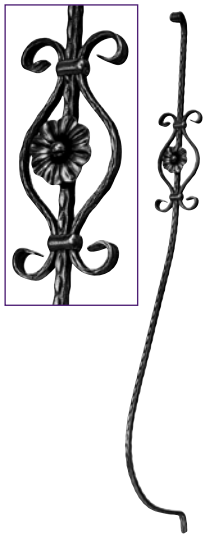
Art. 1269/2 □ 12 x 12 mm 110 x 1500 mm
